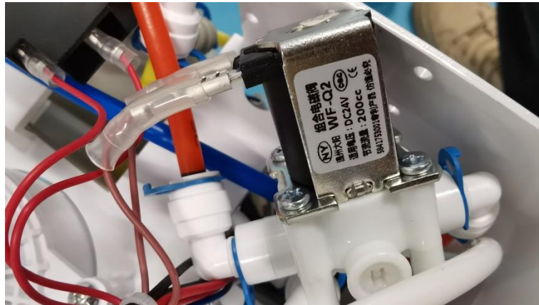
ER0001-3 (组合电磁阀)
